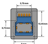
USB 3.0 B
