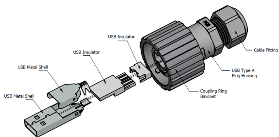
USB 2.0 male
