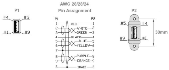
USB 3.0 A
