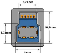
USB 3.0 B
